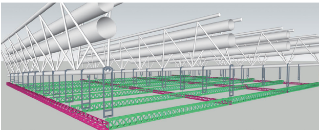
Schematic Diagram of the second-floor basic structure
